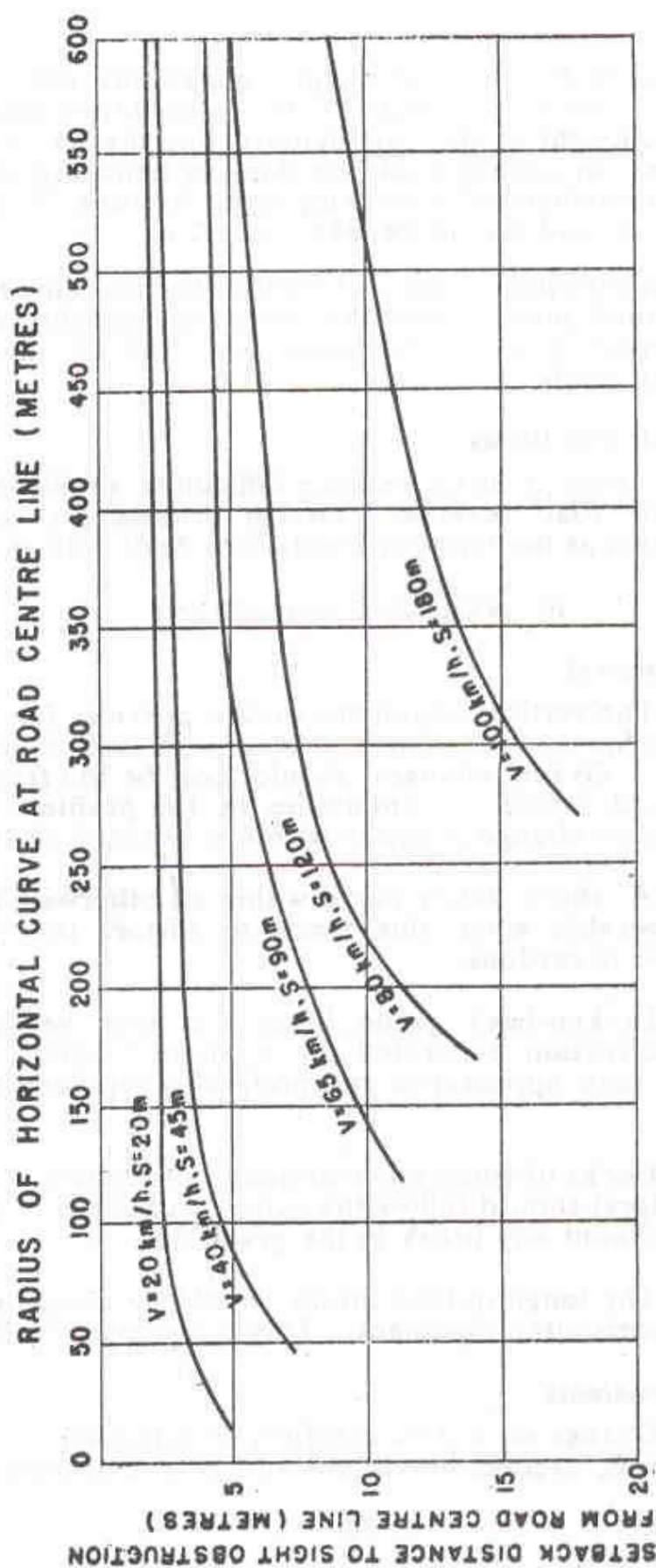
Fig. 4. Minimum set-back distance required at horizontal curves for safe stopping sight distance
