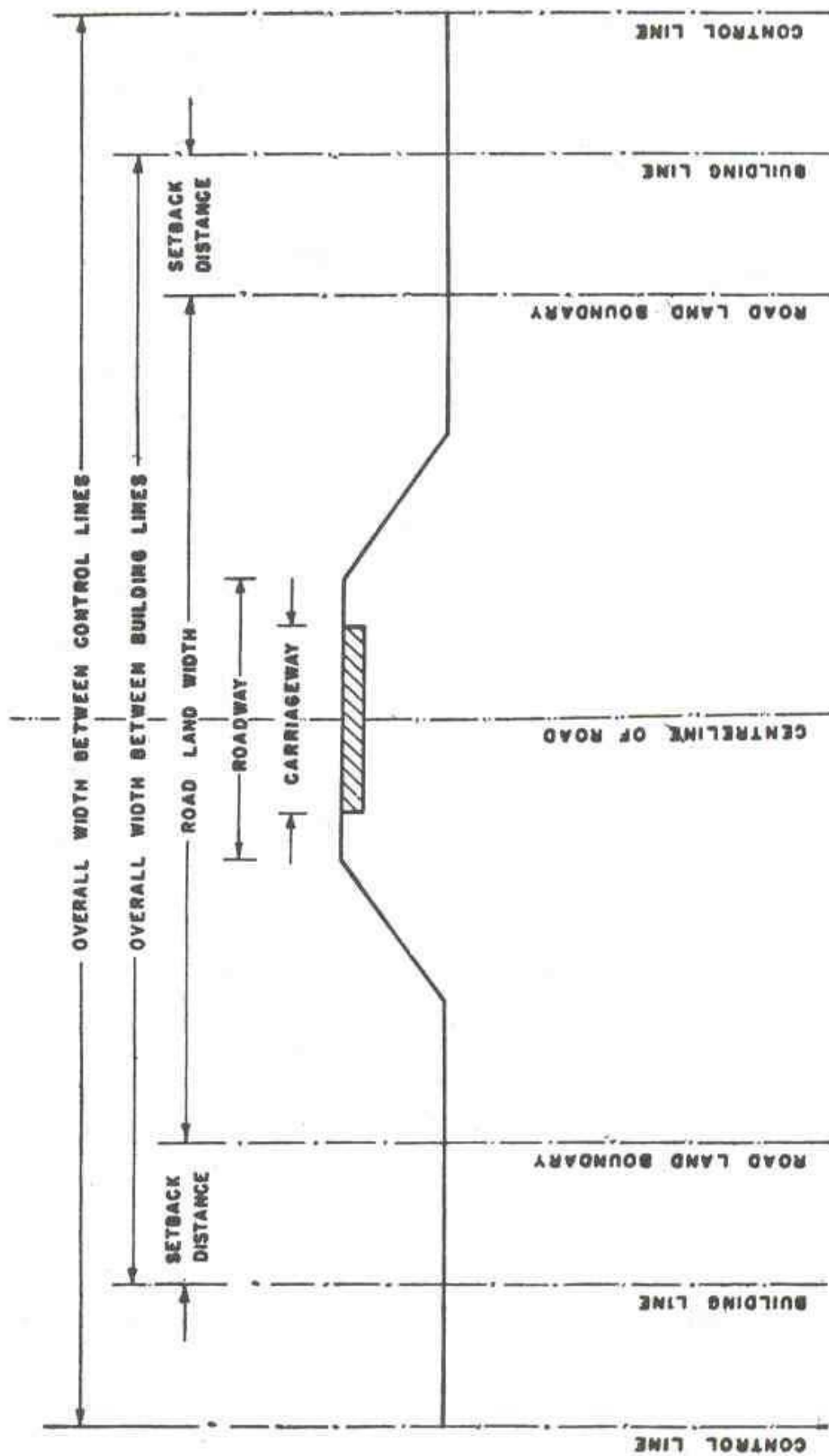
Fig. 1. Road land boundary, building lines and control lines
