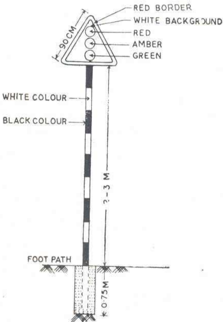
Fig. 2. Signal ahead sign
