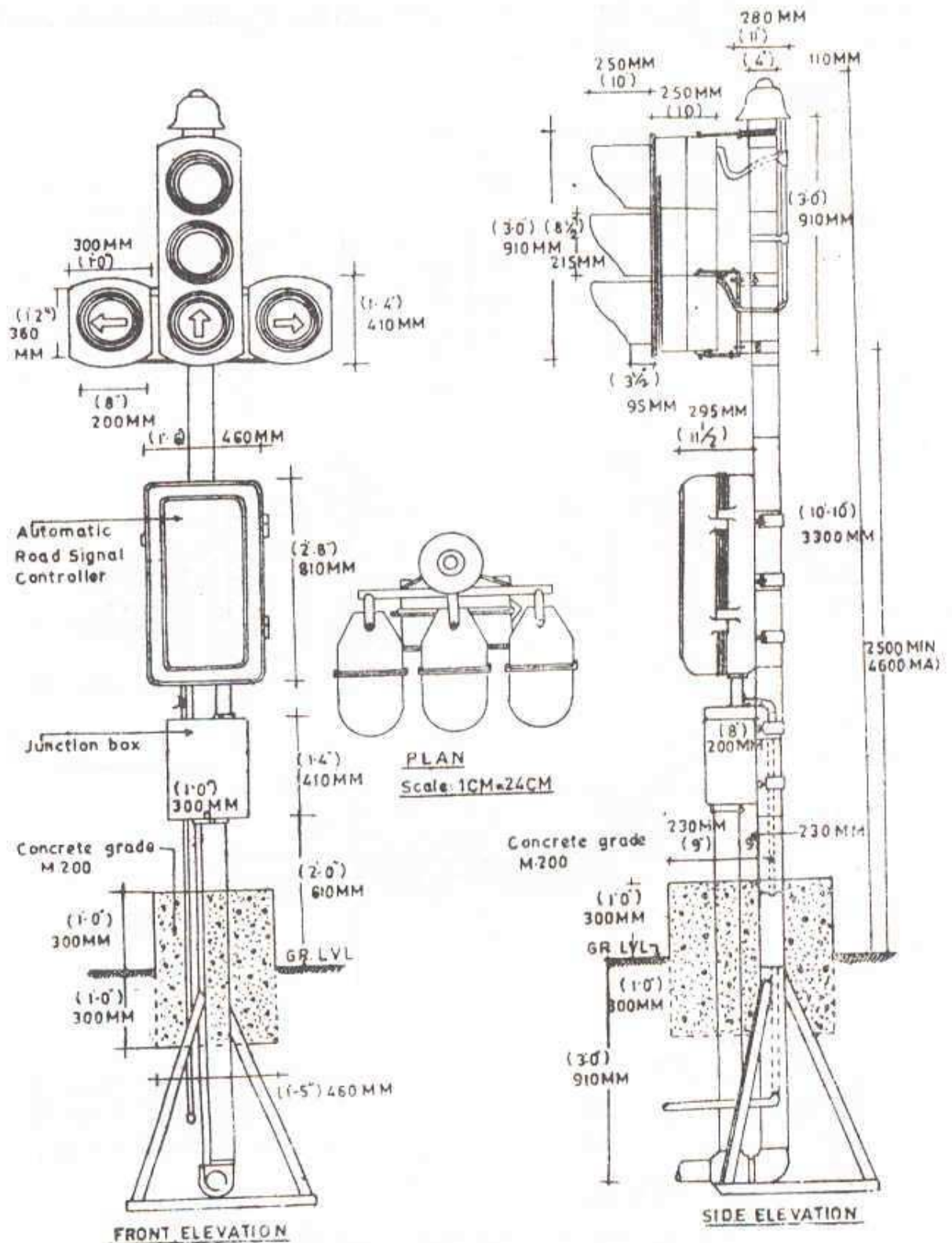
Fig. 4. Typical foundation details of signal pole
