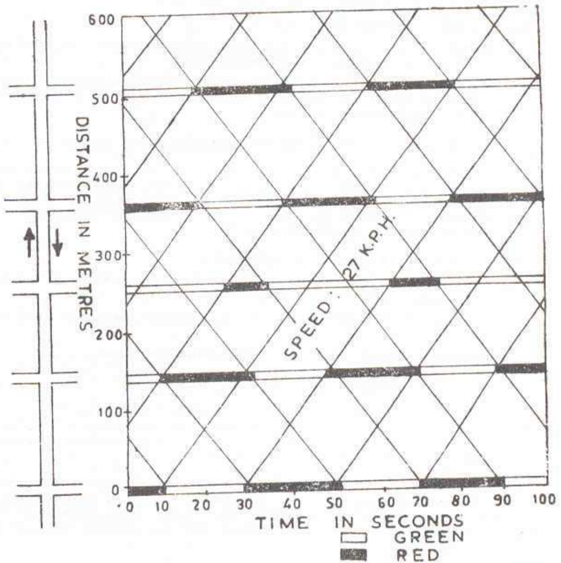
Fig. 8. Typical time and distance diagram for one way streets with linked signals
