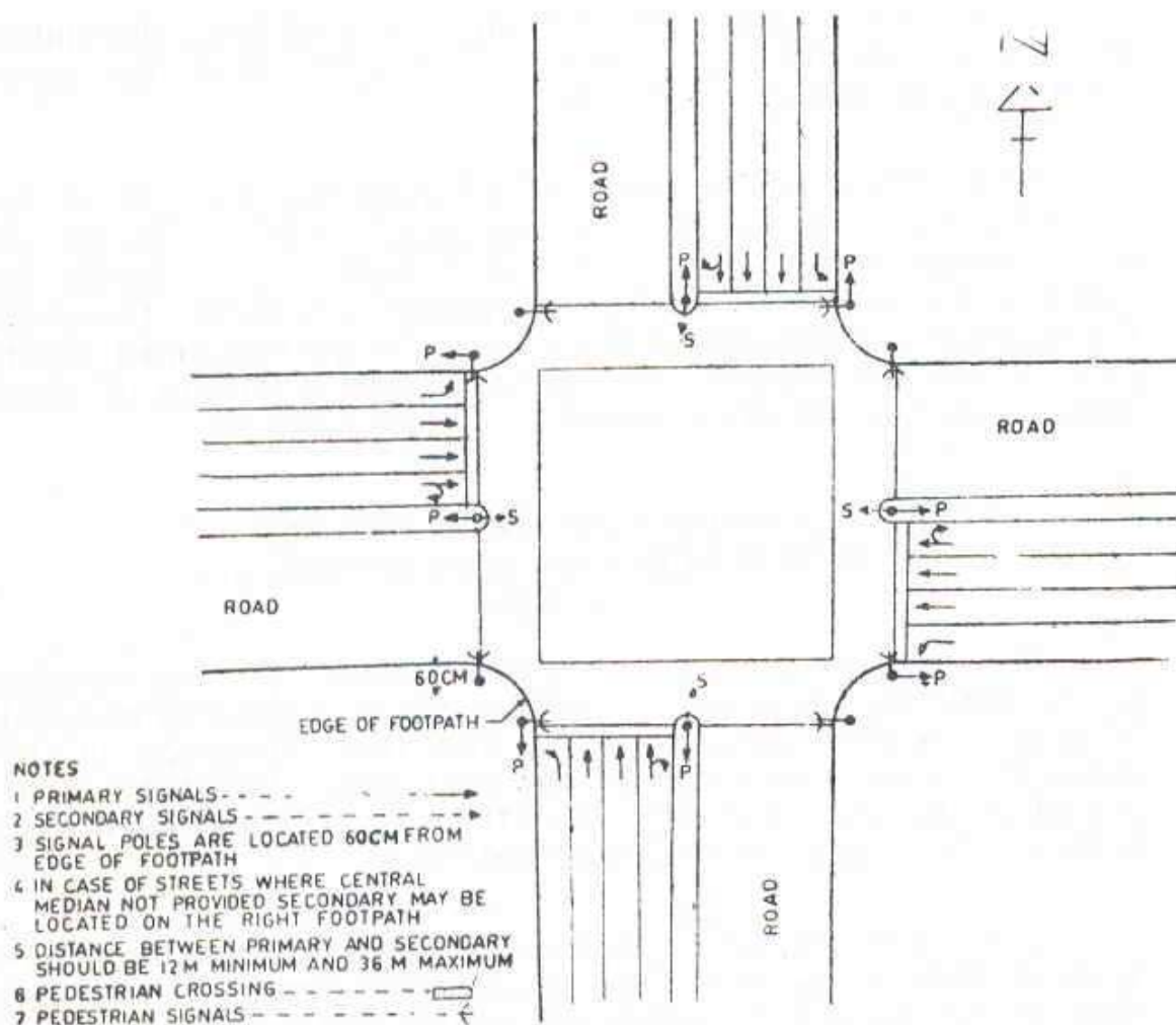
Fig. 3. Transverse location of signal supports
