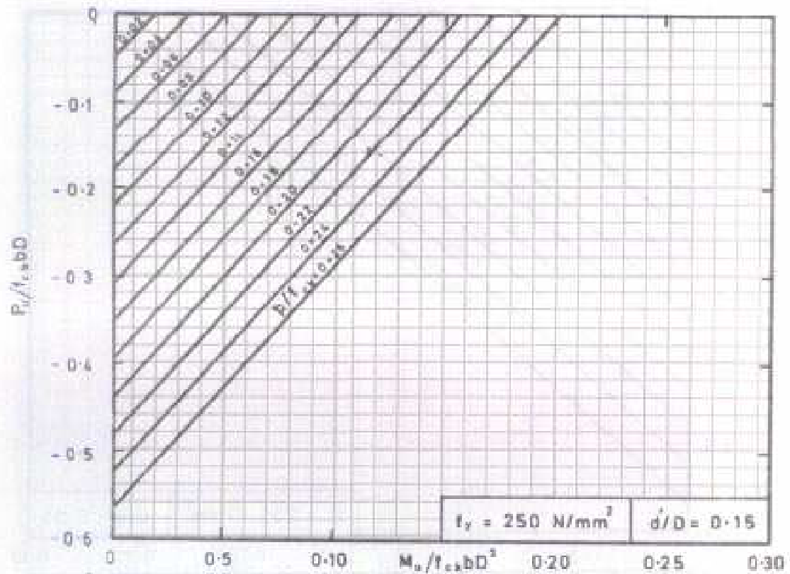
Chart 66 TENSION WITH BENDING — Rectangular Section — Reinforcement Distributed Equally on Two Sides
