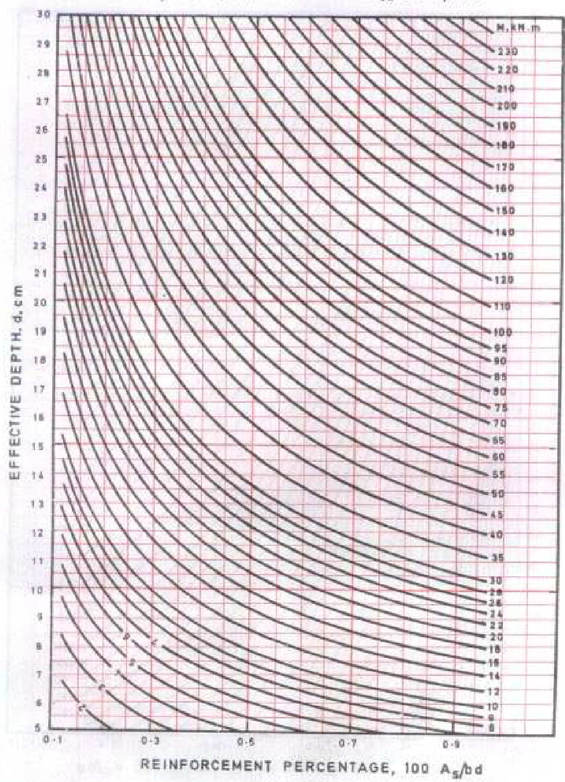
Chart 13 FLEXURE — Singly Reinforced Section Moment of Resistance kN.m per Metre Width
