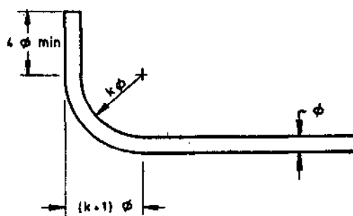
STANDARD 90° BEND
